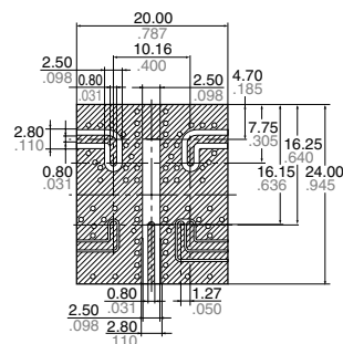
PC board for correction Dimensions (mm inch)
