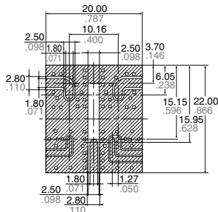
PC board for correction Dimensions (mm inch)
