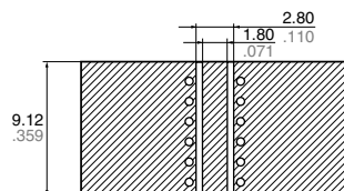
PC board for correction Dimensions (mm inch)
