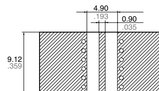
PC board for correction Dimensions (mm inch)
